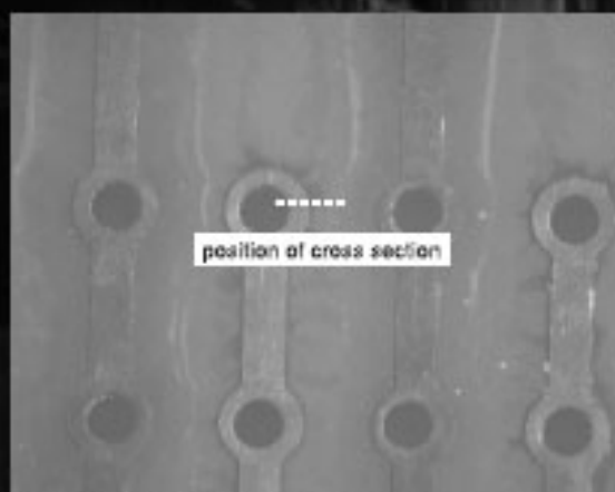
Comb shape copper electrode
