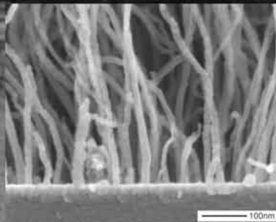
Carbon Nanotube
