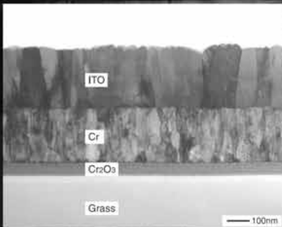
Cross section of glass base for liquid crystal display
