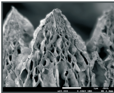
Graphene (80V)
